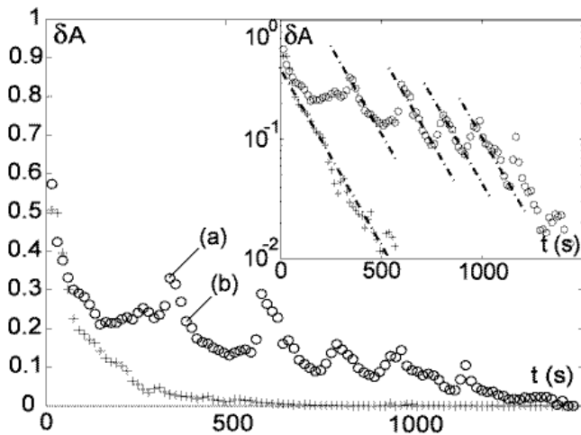
Fig. 3. The mobile volume fraction evolution \delta A(t) for two different realizations at similar pile slopes: (o) \theta = 15^\circ ; (+) \theta = 16.5^\circ . Inset is the log-lin plot of the same data. Notice the exponential decay rate, which is identical in the monotonous case (+) and in the intermittent case (o).
